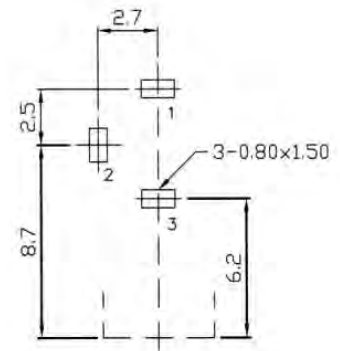
P.C.B. LAYOUT(±0.1) (BOTTOM VIEW)
